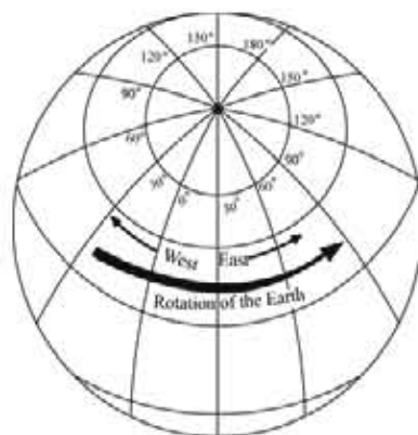
Figure 3.5: Earth's Rotation from West to East
