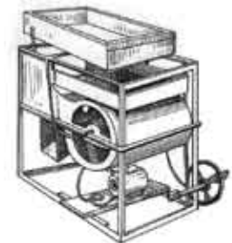
Figure : BARI crop winnower
