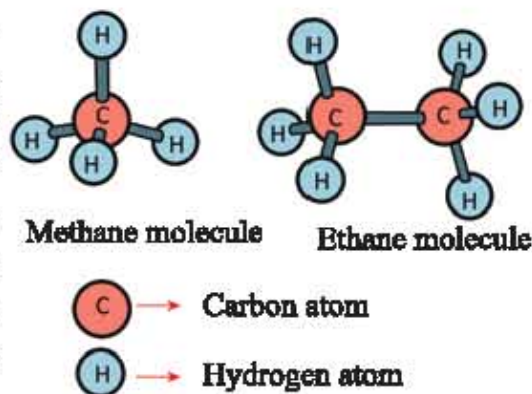
Fig 11.03: Methane and Ethane.
