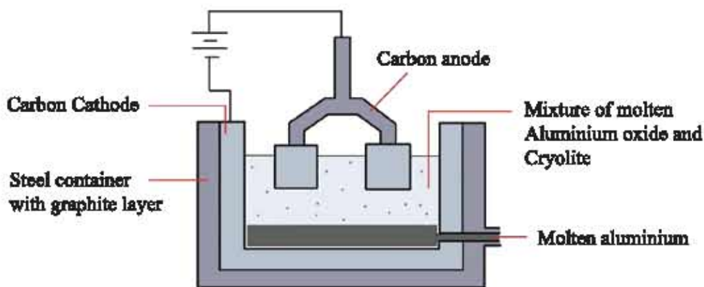
Fig10.07: Aluminium Extraction.
