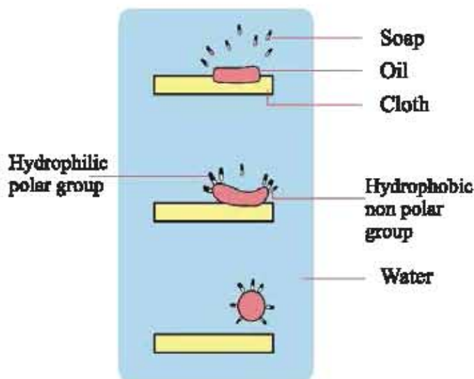
Fig 12.02: Cleaning Mechanism with Soap or Detergent.
