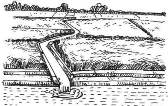
Fig-2.7: Water drainage by permanent furrow
