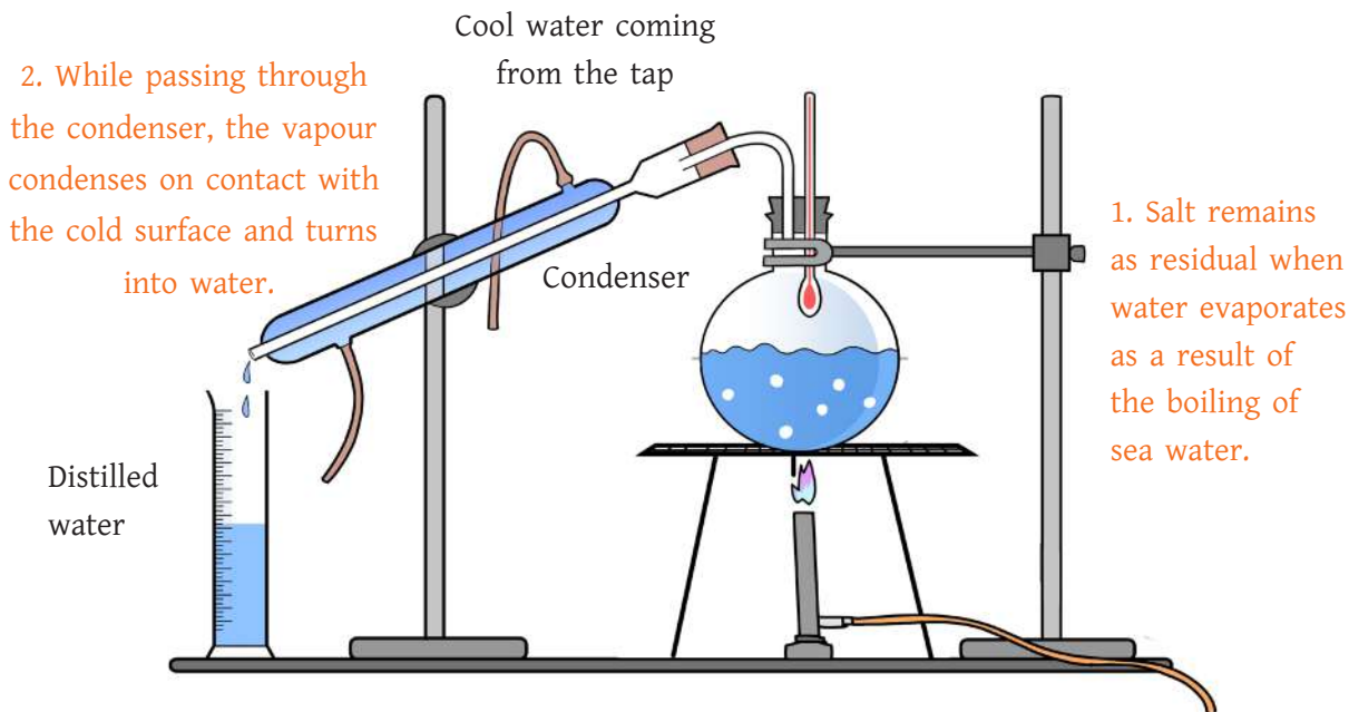
Image: Distillation method
