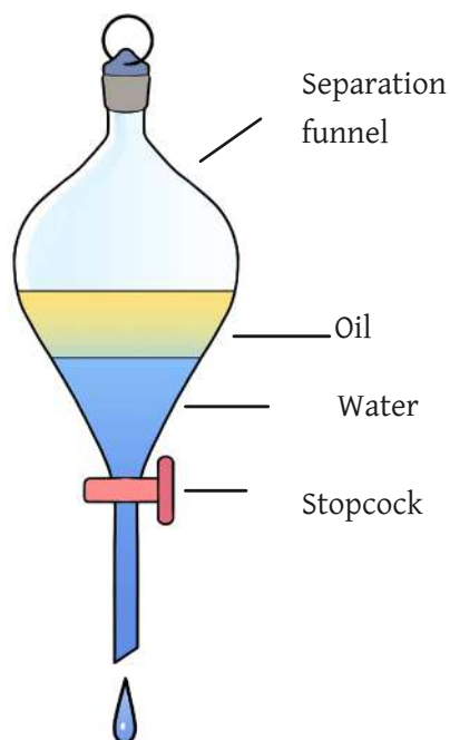
Image: Separation of water and oil by separation method (2)
