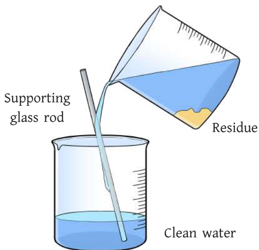
Image: Separation of sand and water by separation method
